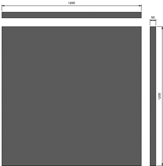
SOUND REDUCTION SYSTEMS SONATA VARIO HIGH PERFORMANCE DECORATIVE RAFT ABSORBER 1200 x 1200 x 50mm
