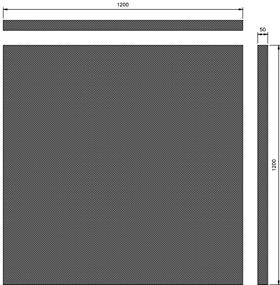
SOUND REDUCTION SYSTEMS SONATA AURIO HIGH PERFORMANCE DECORATIVE BONDED ABSORBER 1200 x 1200 x 50mm
