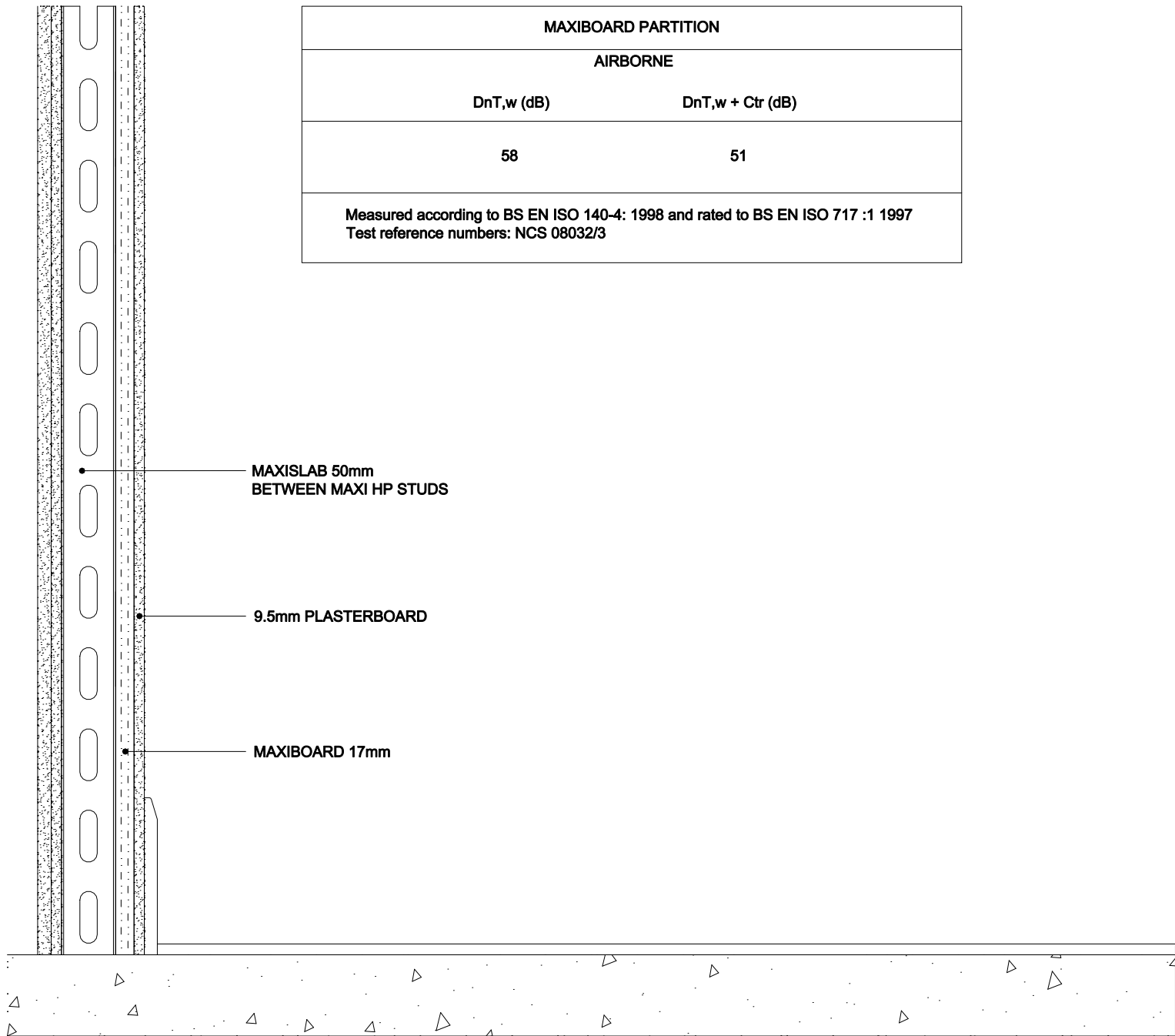
SOUND REDUCTION SYSTEMS MAXIBOARD HP PARTITION WALL HIGH PERFORMANCE
