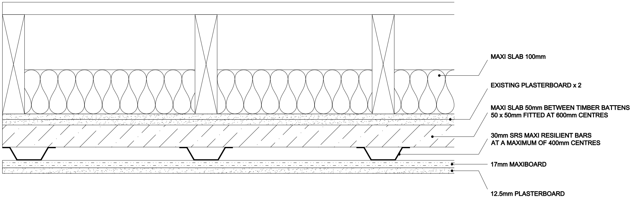
SOUND REDUCTION SYSTEMS MAXI DROPPED CEILING SYSTEM 1/2 HOUR FIRE RATED
