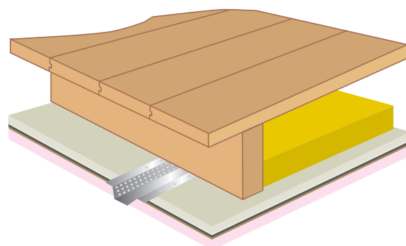
section through Maxi 60 ceiling
