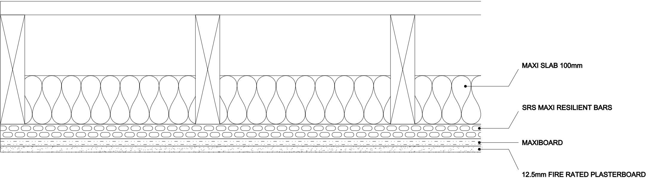
SOUND REDUCTION SYSTEMS MAXI 60 CEILING 1 HOUR FIRE RATED
